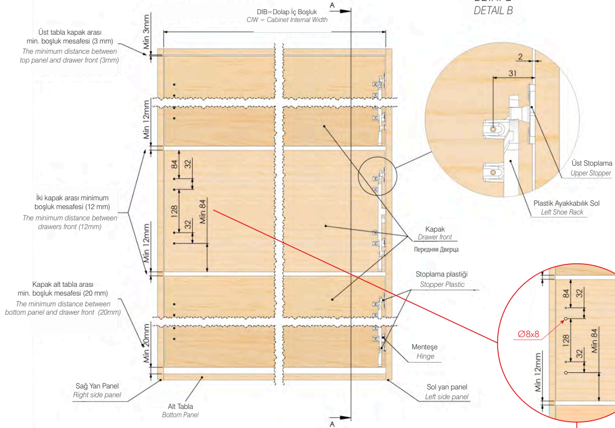
Pimli versiyon Version with pin
