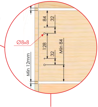
Pimli versiyon Version with pin
