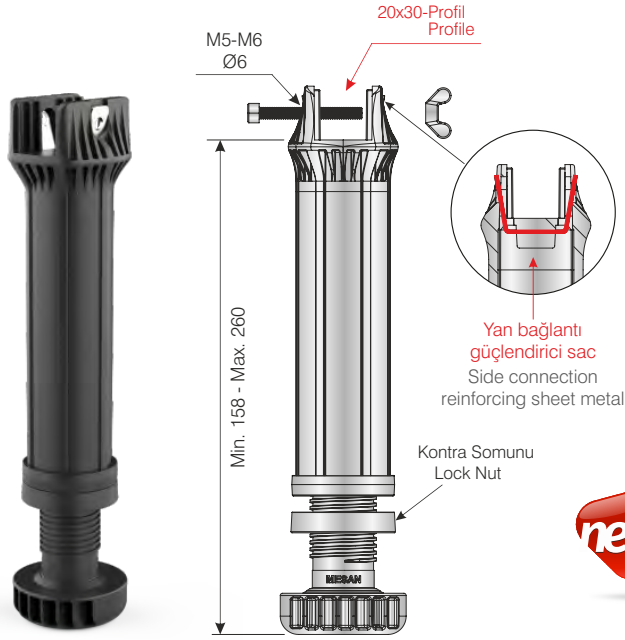
104-01-96 20 x 30 mm Profil 20 x 30 mm Profile
