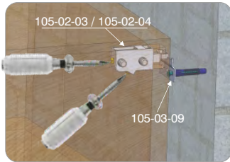
105-02-03 Sol / Left 105-02-04 Sağ / Right
