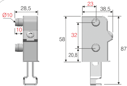
105-02-03 Sol / Left 105-02-04 Sağ / Right
