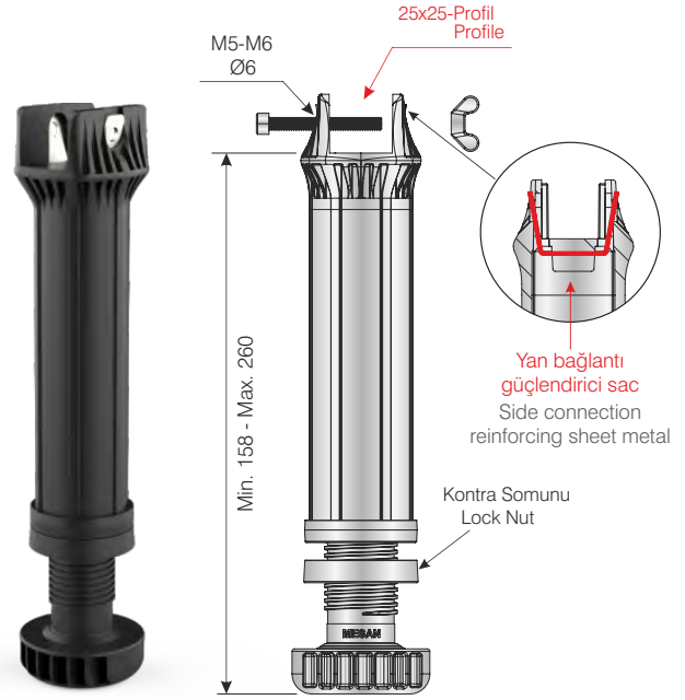
104-01-95 25 x 25 mm Profil 25 x 25 mm Profile
