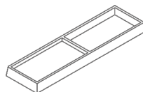
S7 TRAY (COUNTERTOP) / BANDEJA (S/ENCIMERA) GLASS / CRISTAL Ref. 129393 A: 288 mm. B: 22 mm. C: 82 mm.
