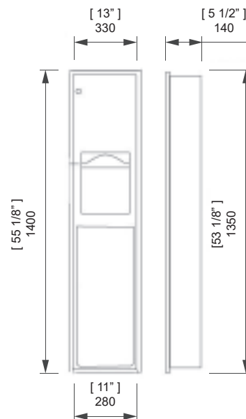
SATIN STAINLESS STEEL Ref. 174867
