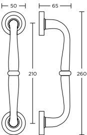
ΛΑΒΗ ΕΞΩΘΥΡΑΣ PULL HANDLE
