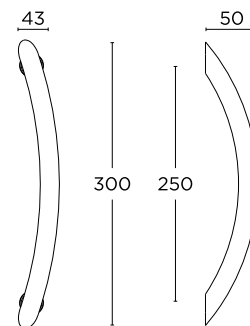
ΛΟΞΗ ΛΑΒΗ ΕΞΩΠΟΡΤΑΣ CURVED OUTDOOR PULL HANDLE
