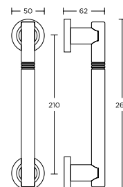
ΛΑΒΗ ΕΞΘΥΡΑΣ PULL HANDLE
