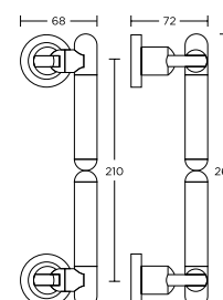
ΛΑΒΗ ΕΞΩΘΥΡΑΣ PULL HANDLE
