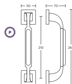
ΛΑΒΗ ΕΞΩΘΥΡΑΣ PULL HANDLE
