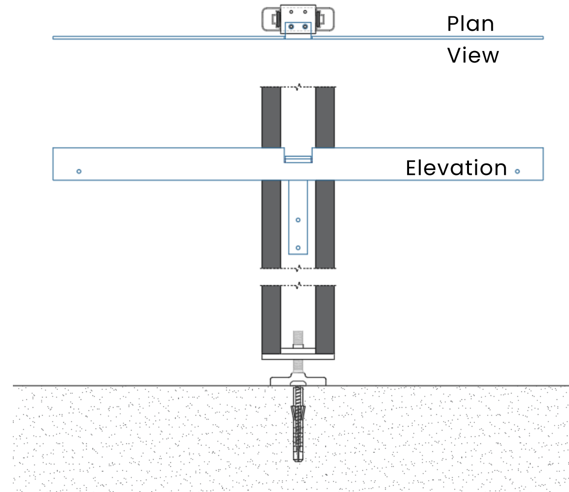
Connector with Hanger
