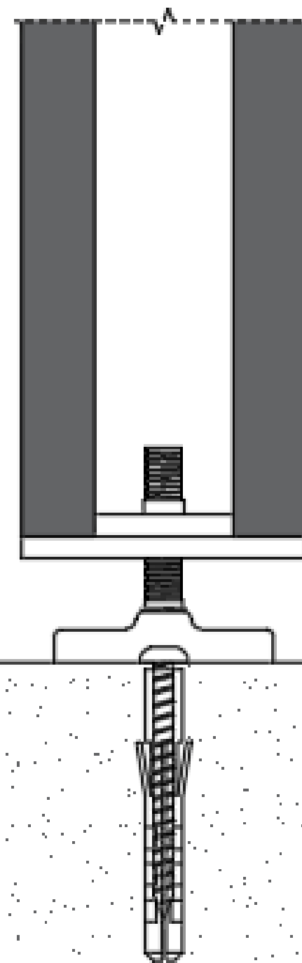
• Side View : Showing the assembly of aluminium profiles fixed to the support system
