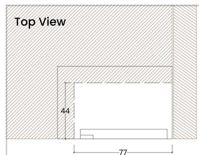
Hinge Installation Bracket
