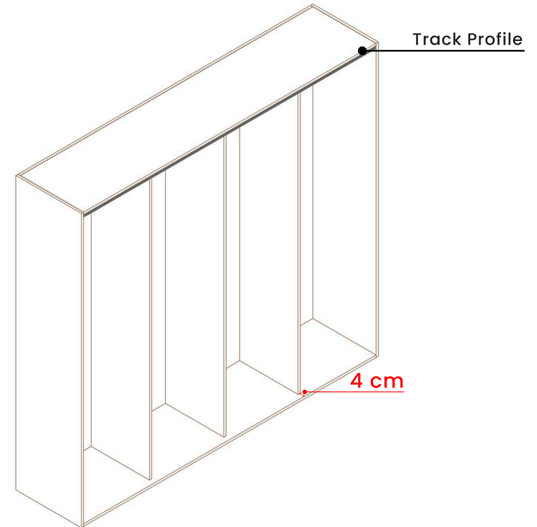
Isometric view
