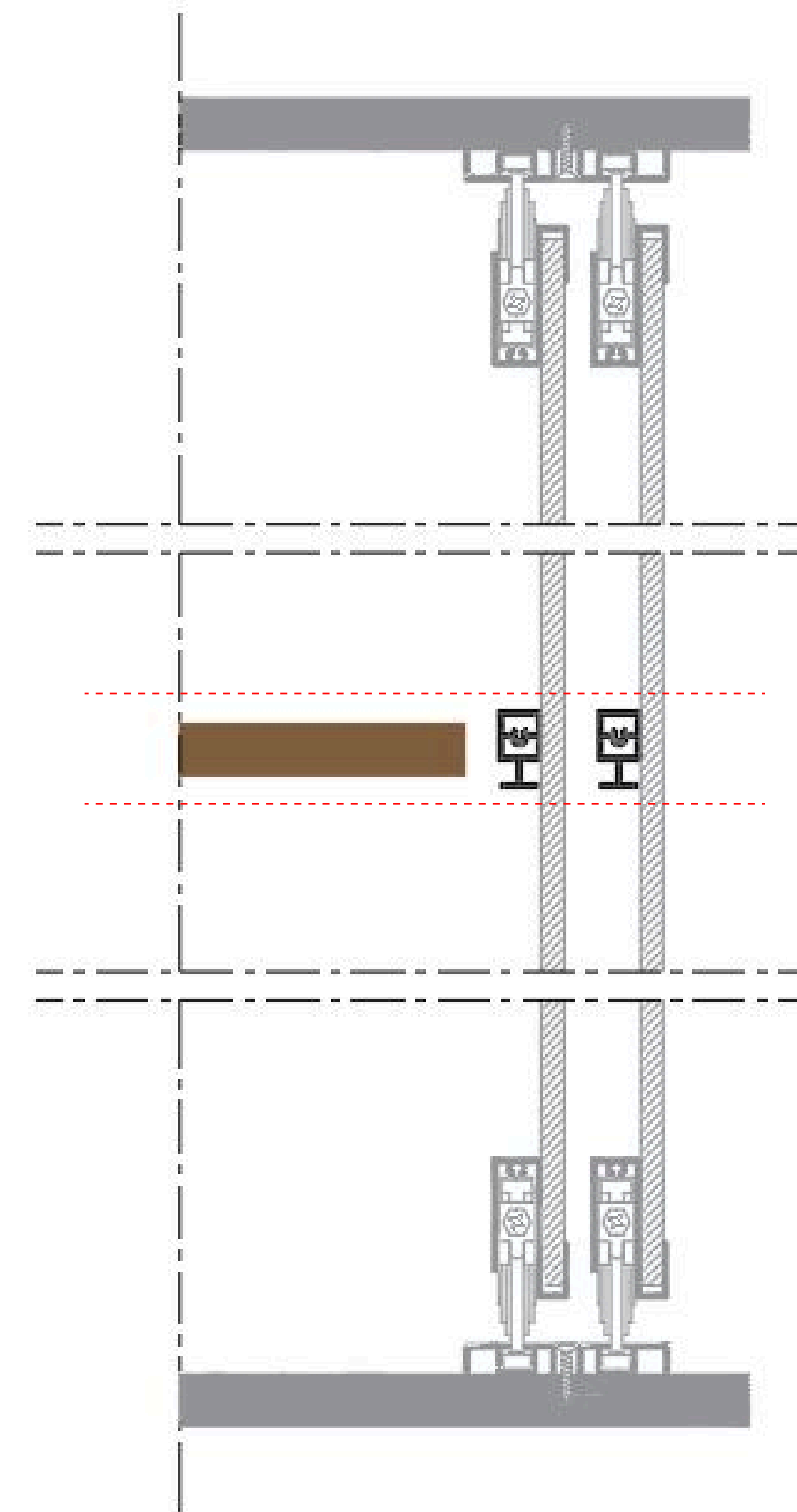
Section View – Closet Installation
