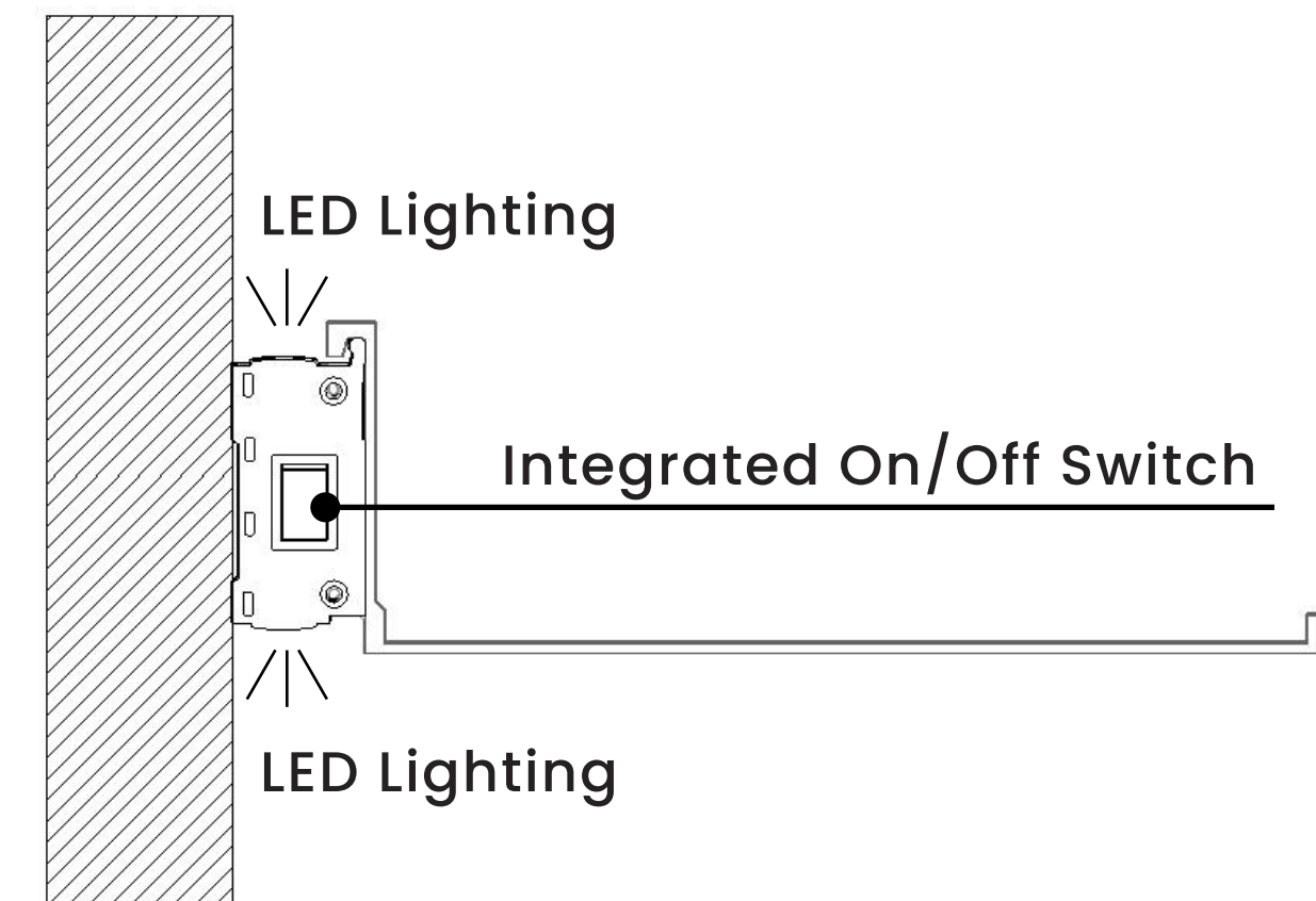
• Shelf With Back Profile Assembly
